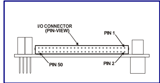
Figure 2. 50-Pin System I/O Connector
