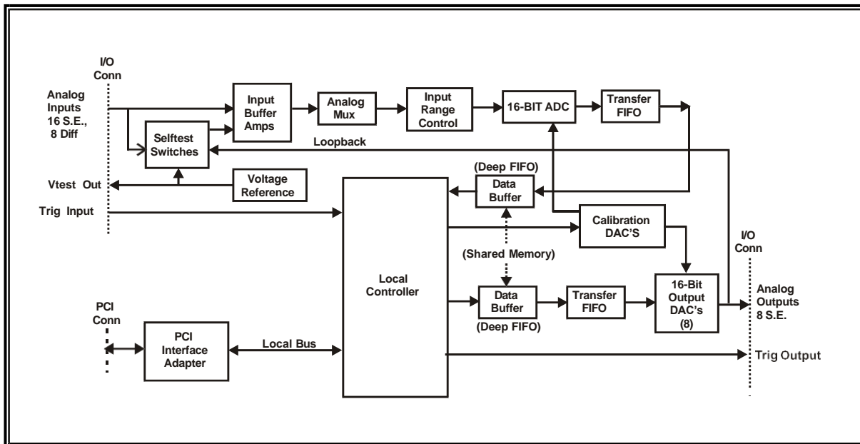
Figure 1. 16AIO168; Functional Organization
